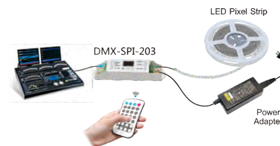
6.2 Connection with DMX console:
