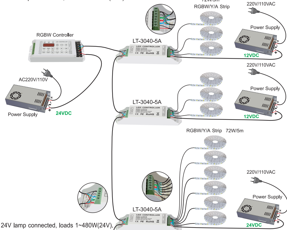
A. 12V lamp connected, loads 1~240W(12V).
